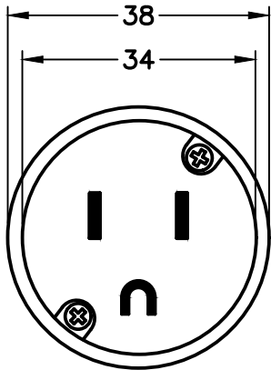
NEMA 5-15 PLUG FRONT VIEW
